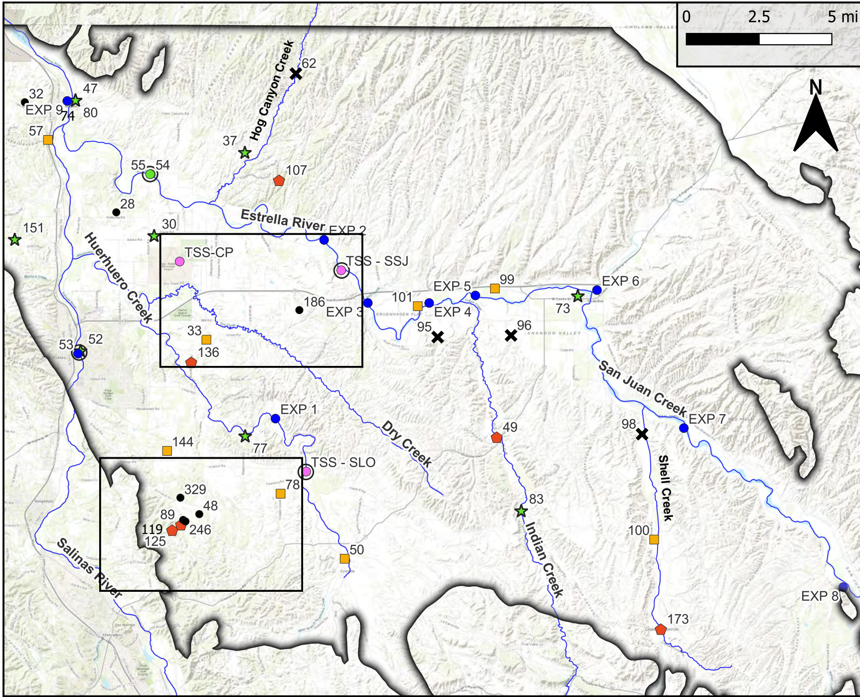
Figure 1 Telemetry Installation Status for the Expanded Monitoring Well Network
